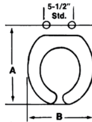
SEAT ATTACHING HOLES
